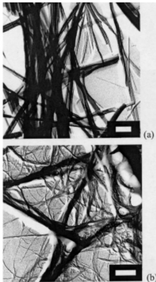
Figure 1. Electron micrographs of p -xylene gels of 3 (a) and 4 (b) (10 mg/mL, Pt shadow 45°, bar = 1 \mu\text{m} )
